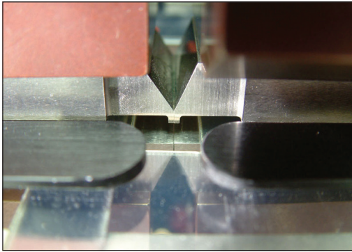
Z-Span™ anvils and jaw tips
